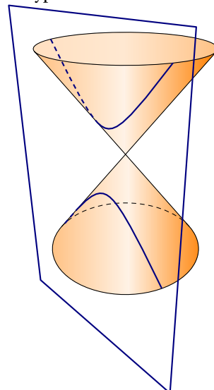
FIGURE 14 : Hyperbole : intersection cône - plan
