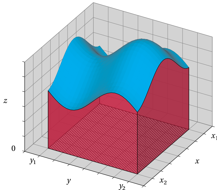
FIGURE 41 : Volume correspondant à \int_{x_1}^{x_2} \int_{y_1}^{y_2} f(x,y) dx dy
