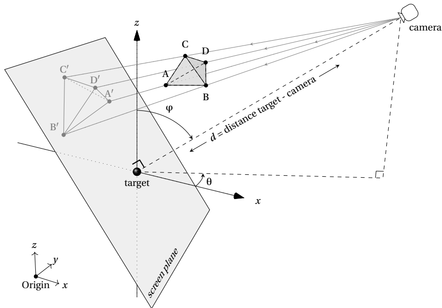
FIGURE 4 : Projection centrale
