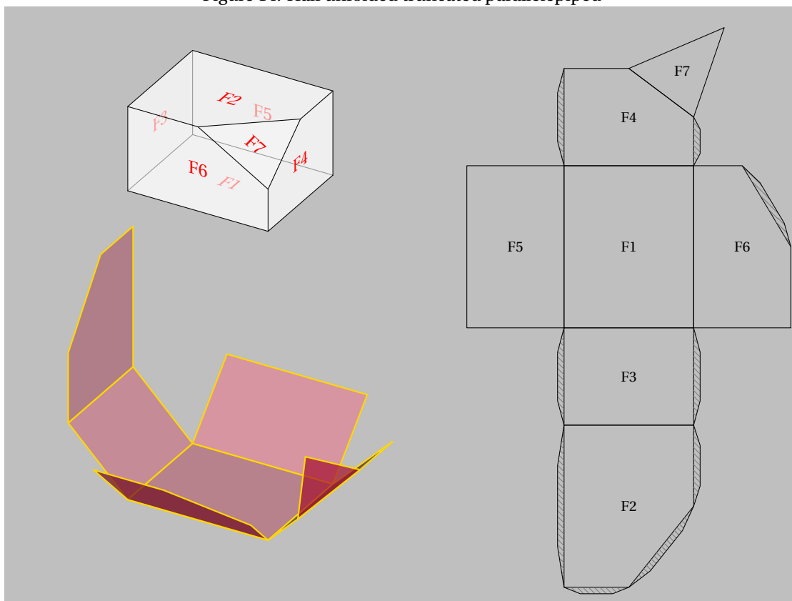
Figure 14: Half unfolded truncated parallelepiped
