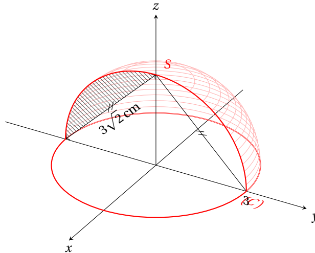
Figure 30: 3D Decorations
