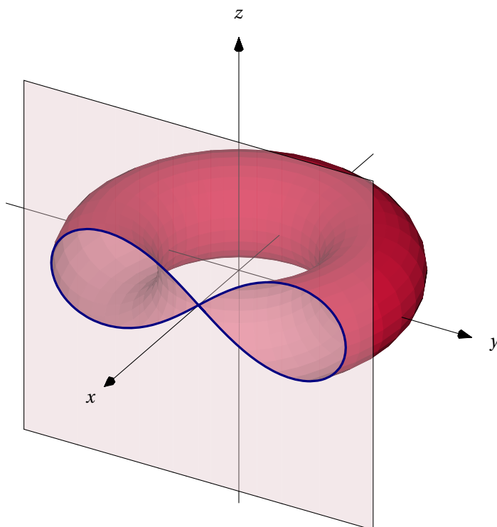
Figure 32: Torus and lemniscate
