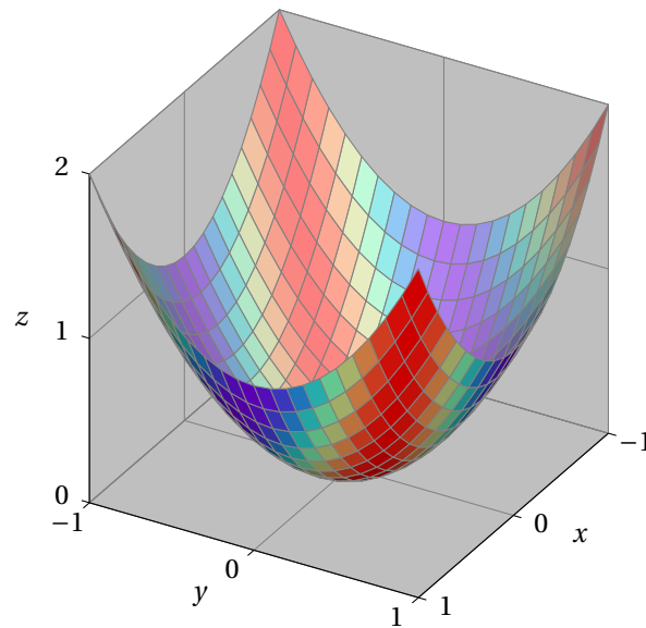
Figure 22: The function ld.read_table3d()
