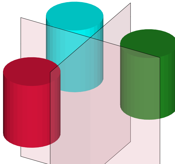
Figure 31: Example with addWall (the two transparent pink facets are normally invisible)
