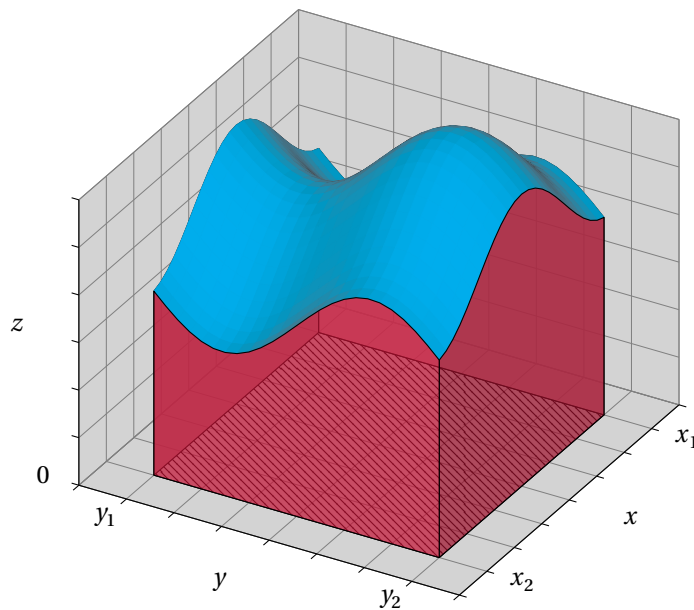
Figure 41: Volume corresponding to \int_{x_1}^{x_2} \int_{y_1}^{y_2} f(x,y) dx dy
