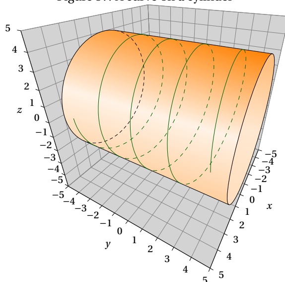
Figure 37: A curve on a cylinder
