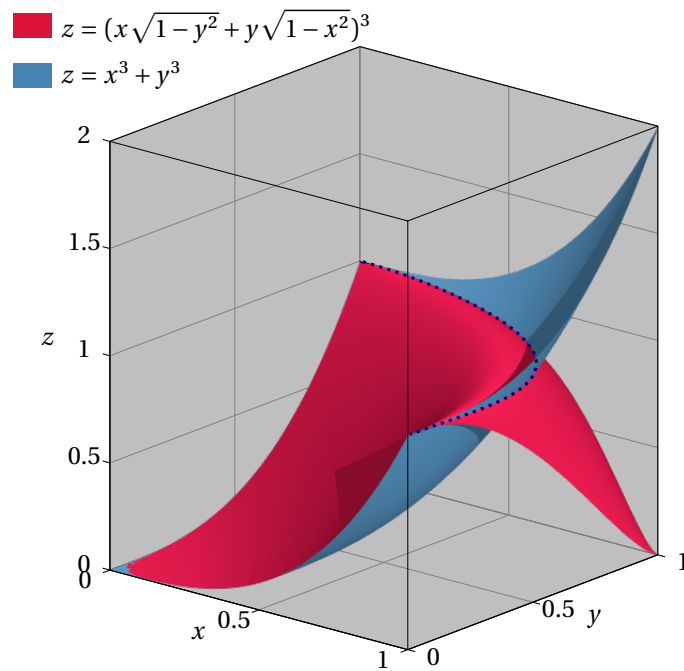
Figure 22: Intersection of two implicit surfaces
