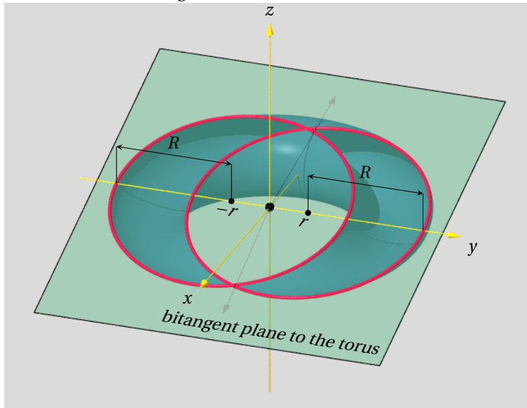
Figure 23: Villarceau circles
