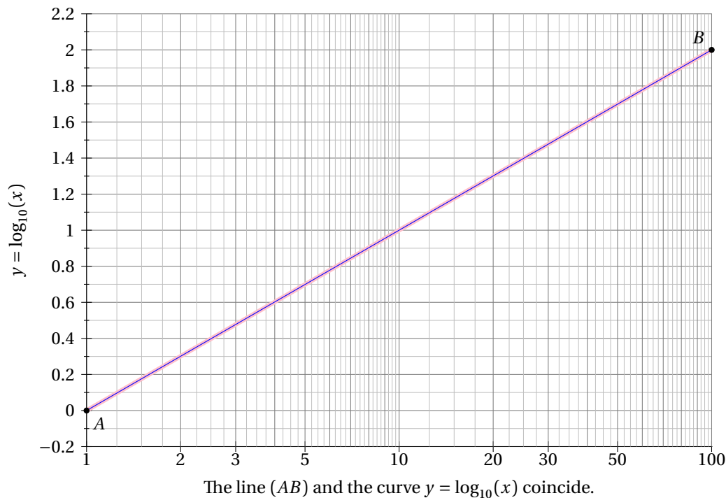
Figure 25: Logarithmic x-axis
