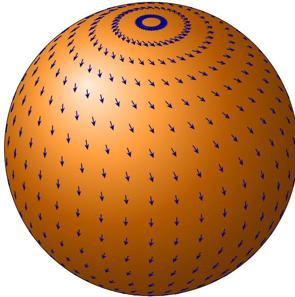
Figure 17: On a sphere
