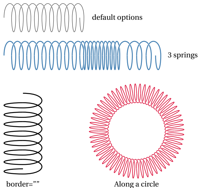
Figure 32: The g:Dcoil2() Method
