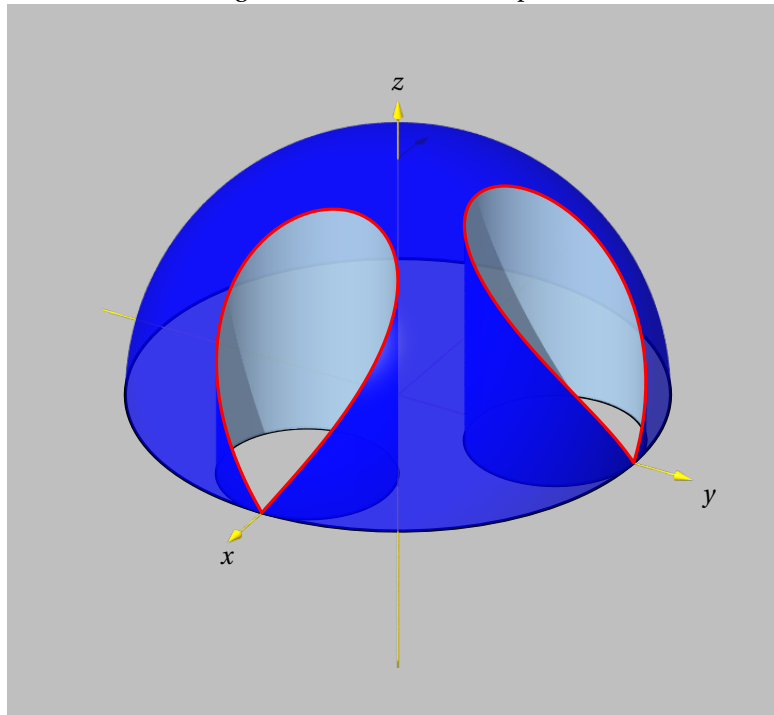
Figure 24: Holes in a hemisphere
