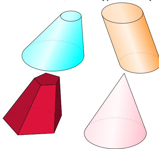
Figure 13: Truncated cone, truncated pyramid, oblique cylinder
