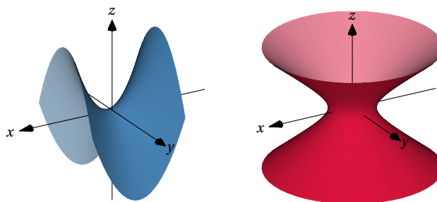
Figure 18: Surfaces using the addwall option
