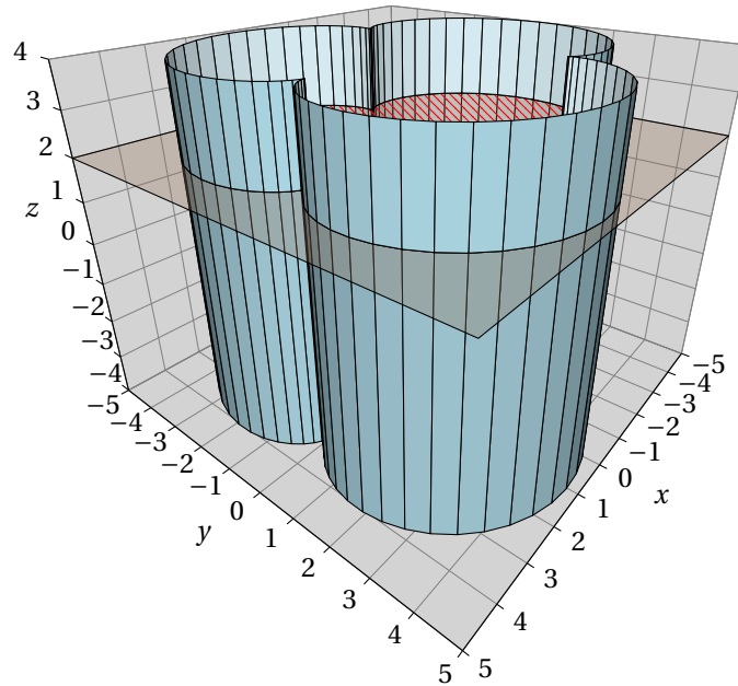
Figure 20: Section of a non-circular cylinder
