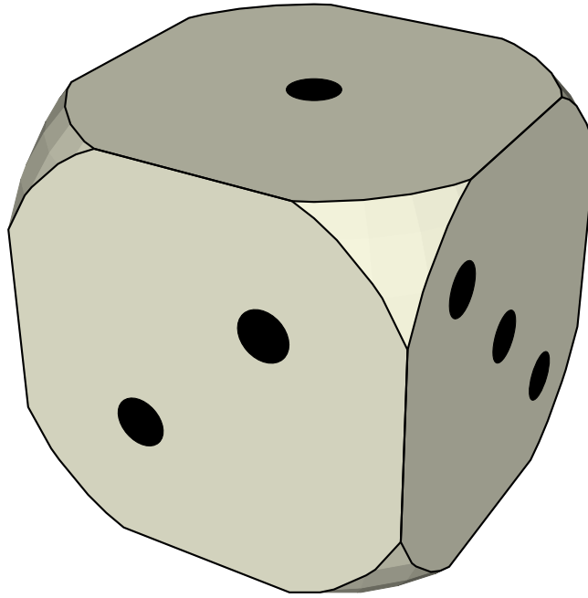
Figure 27: Example with clip3d: constructing a die from a cube and a sphere
