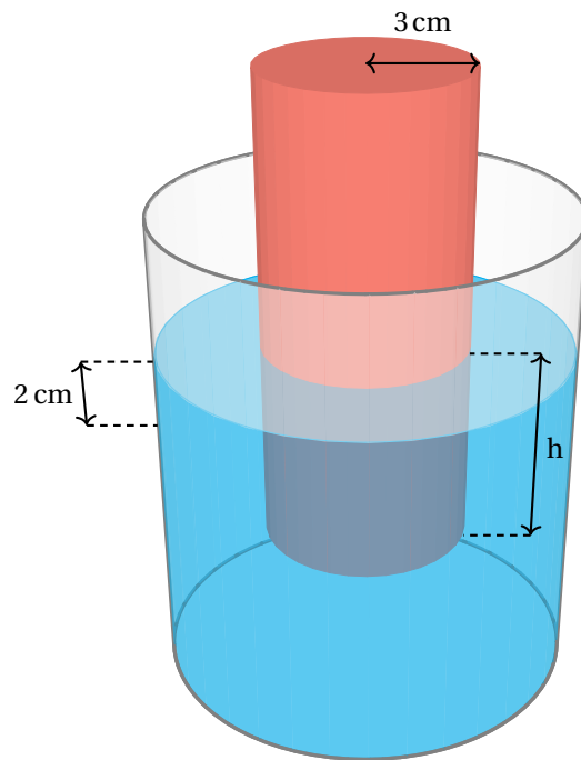
Figure 29: Solid cylinder immersed in water
