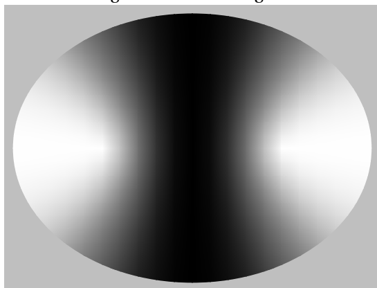
Figure 21: Shaded region
