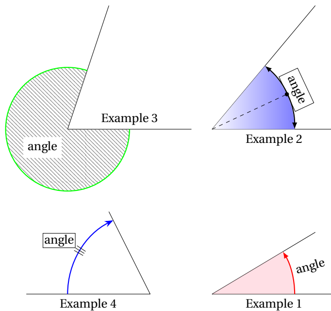
Figure 27: g:Darc() Method
