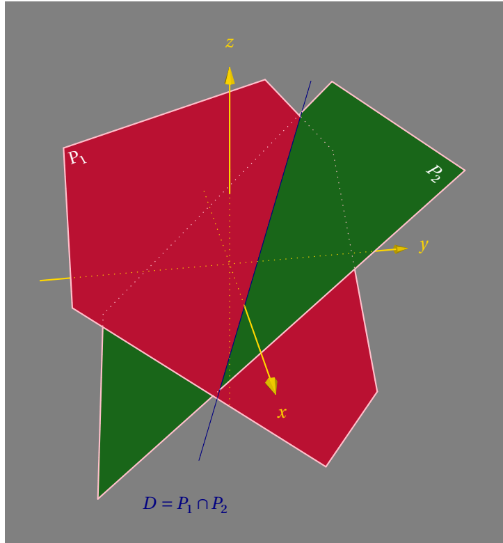
Figure 28: First example with Dscene3d: intersection of two planes
