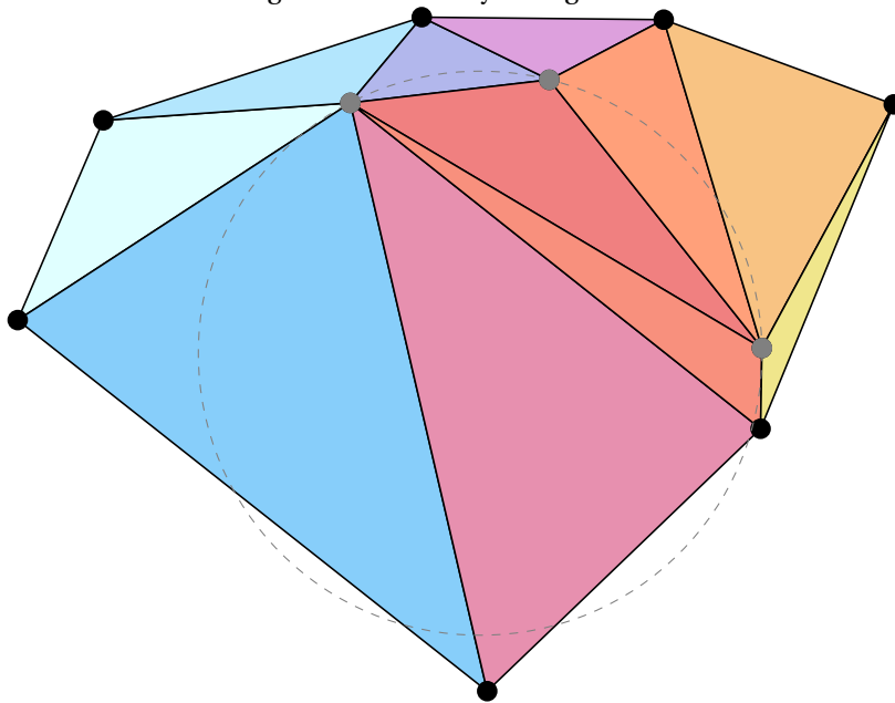
Figure 25: Delaunay Triangulation
