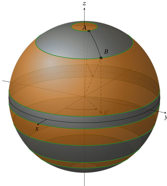
Figure 8: Adding paths
