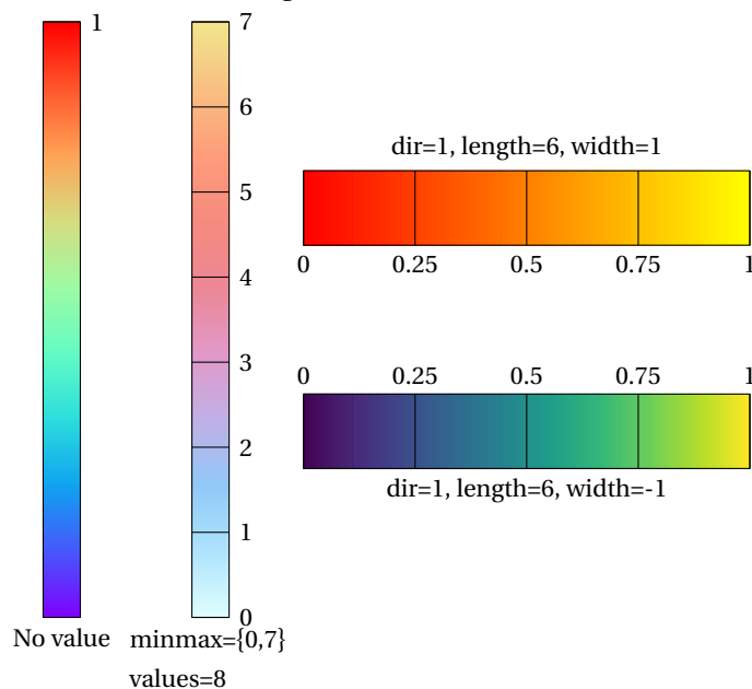
Figure 19: Color bars
