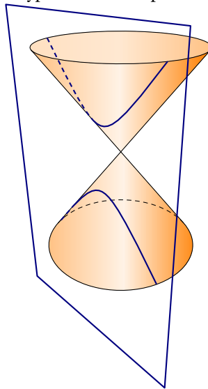
Figure 14: Hyperbola: cone-plane intersection
