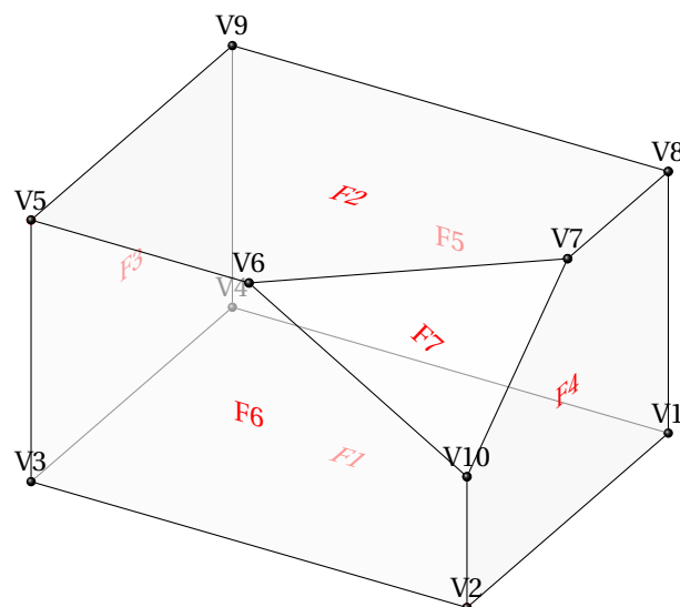
Figure 12: Visualize the faces and vertices of a polyhedron
