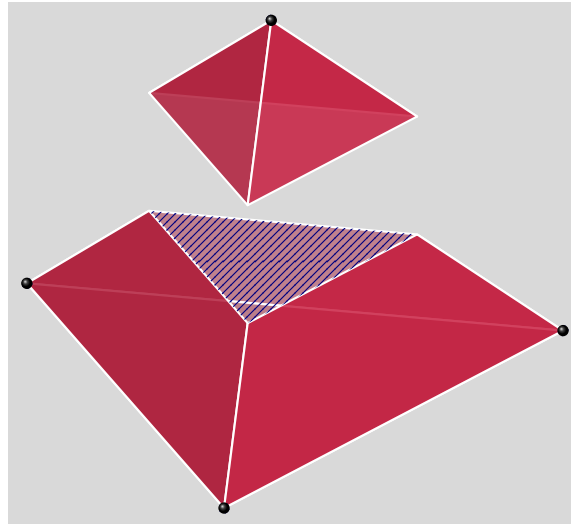
Figure 11: Section of a tetrahedron by a plane
