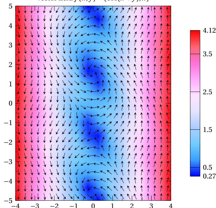
Figure 20: Shaded rectangle vector field f(x,y) = (\cos(x+y), x)
