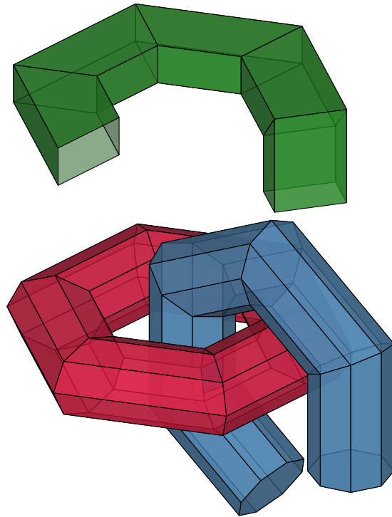
Figure 21: Example with line2tube and section2tube
