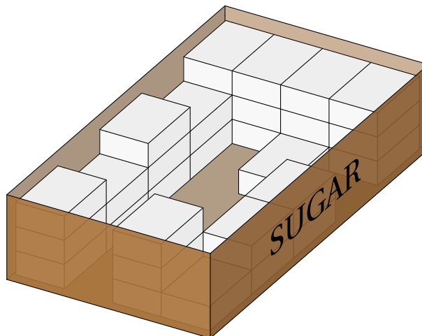
Figure 38: Box of Sugar Cubes
