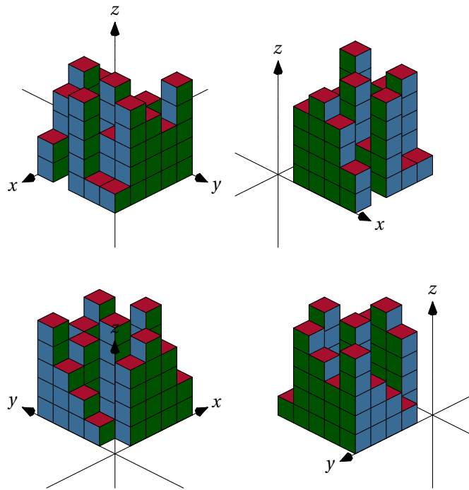
Figure 39: Stack of Cubes
