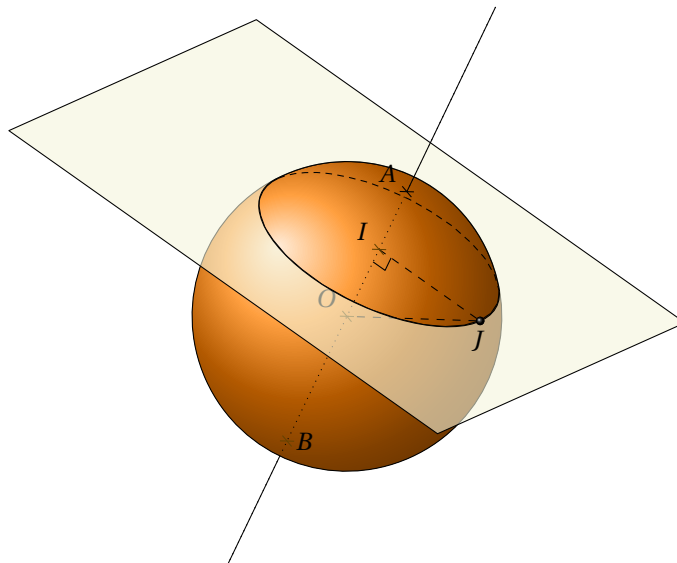
Figure 33: Section of a sphere without Dscene3d()
