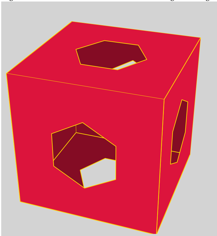
Figure 35: Faces of a cube with holes in it and a regular hexagon
