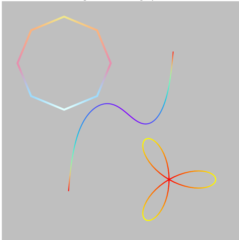
Figure 18: Shaded polyline
