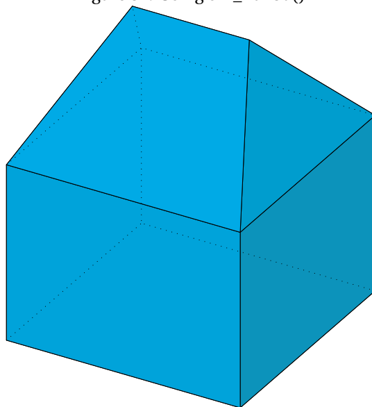
Figure 34: Using cvx_hull3d()
