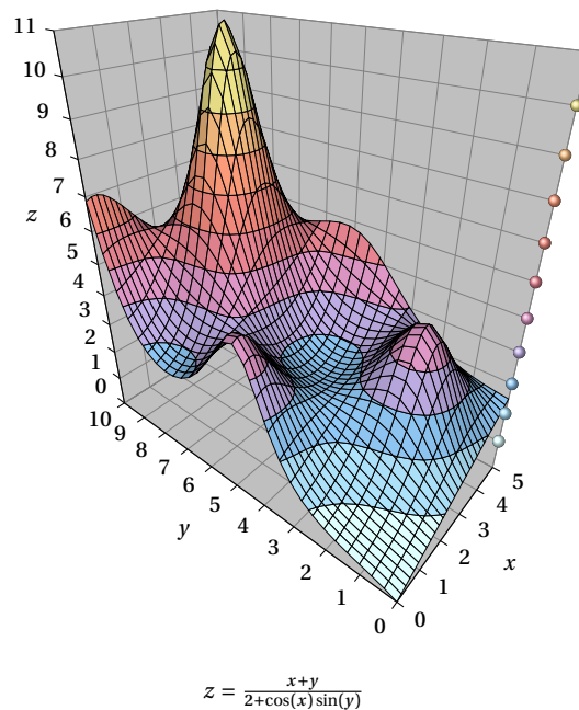
Figure 17: Example of contour lines on a surface
