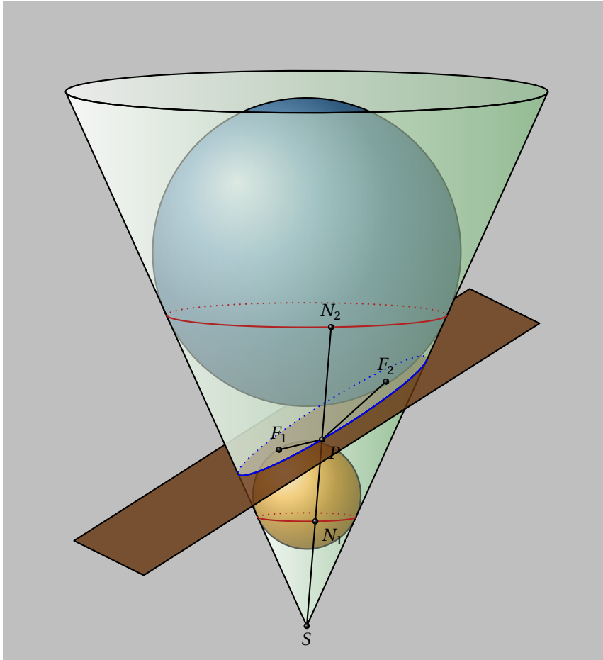
Figure 40: Illustration of Dandelin's Theorem
