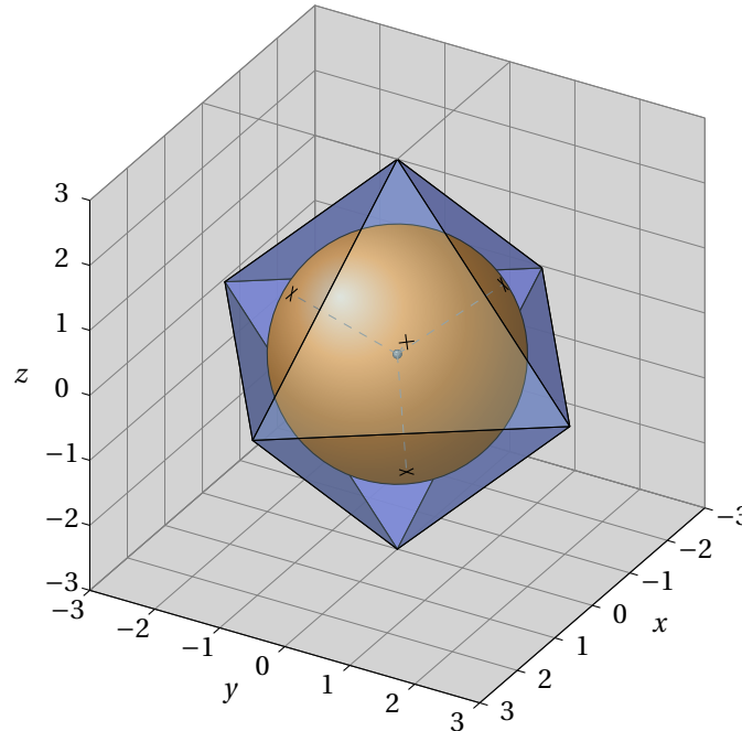
Figure 25: Sphere inscribed in an octahedron with the center projected onto the faces
