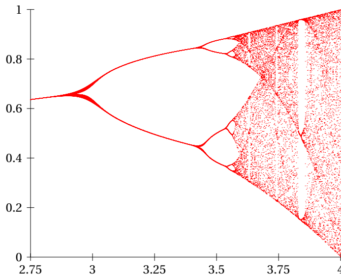
Figure 35: Bifurcation diagram of the sequence u_{u+1} = r u_n (1 - u_n)
