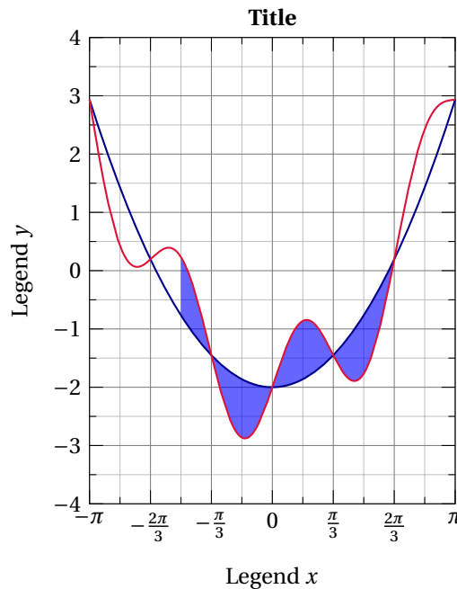
Figure 19: Using Dgradbox
