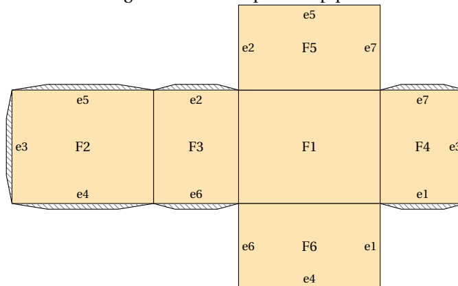
Figure 12: Net of a parallelepiped
