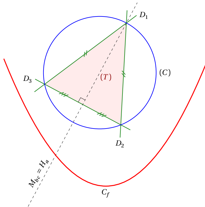
Figure 29: 2D Decorations
