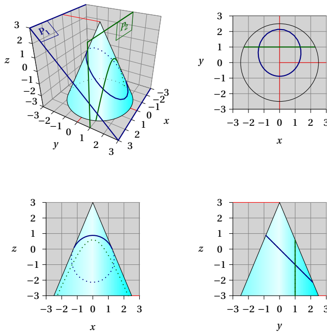
Figure 15: Cone section with multiple views
