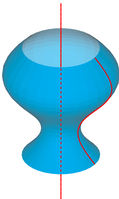
Figure 23: Example with rotcurve
