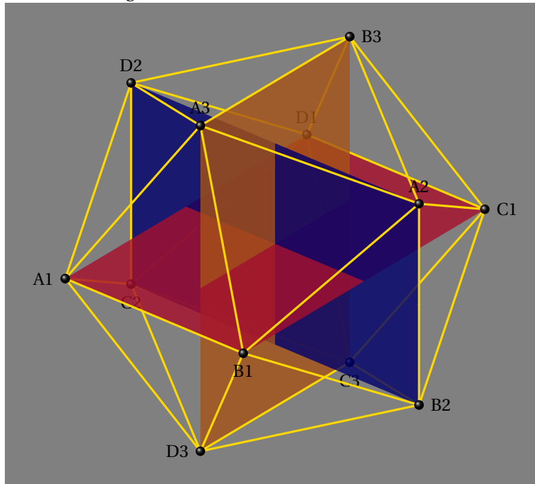
Figure 30: Construction of an icosahedron
