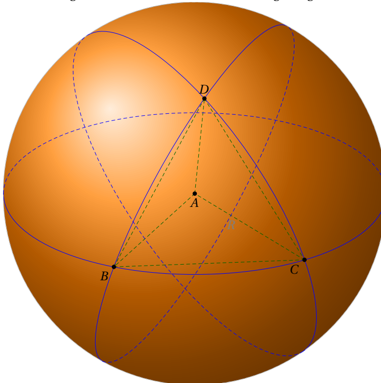
Figure 36: A tetrahedron with fixed edge lengths
