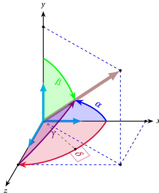
Figure 28: Method g:Darc3d()
