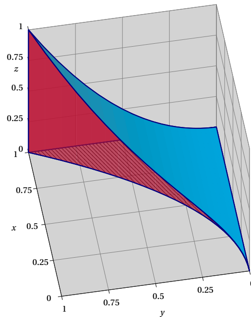
Figure 42: Volume : 0 \leq x \leq 1 ; 0 \leq y \leq x^2 ; 0 \leq z \leq y^2
