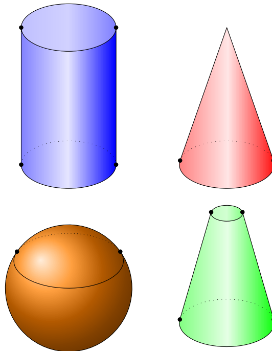
Figure 10: Points of tangency
