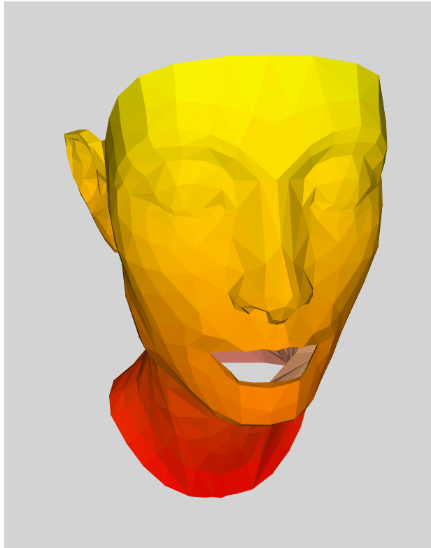
Figure 16: Mask of Nefertiti
