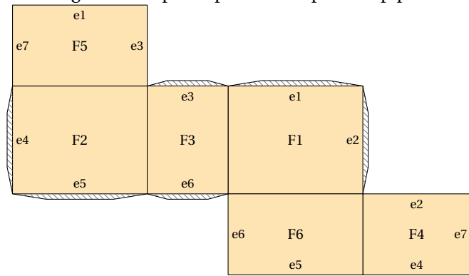
Figure 13: Imposed pattern of a parallelepiped
